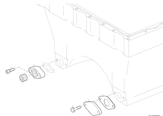
FLANGE OIL PAN 5 SOLID S4000 C23/S83 X00 UPC.06E02 0010
