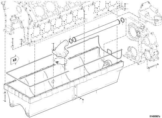
PAN OIL CAST ALUM 16V4000 S83 X00019304 UPC.06E00 1000
